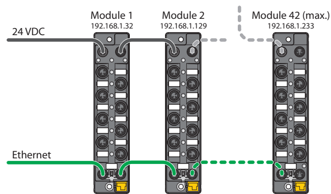
Abb. 7: Daisy-Chain
