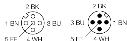
Circuit Diagram
