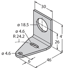
SMBAMS18P
