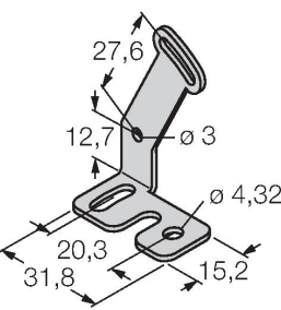
SMBQS18AF 3067467
