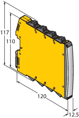
IMX12-DO01-1U-1U-0/24VDC 7580101
