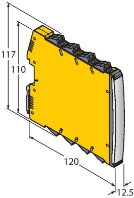
IMX12-DO01-2U-2U-0/24VDC 7580105
