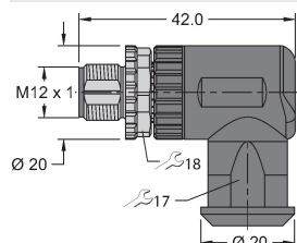
BLANK-LABEL-FOR-CORDSETS-TEL-TXL
